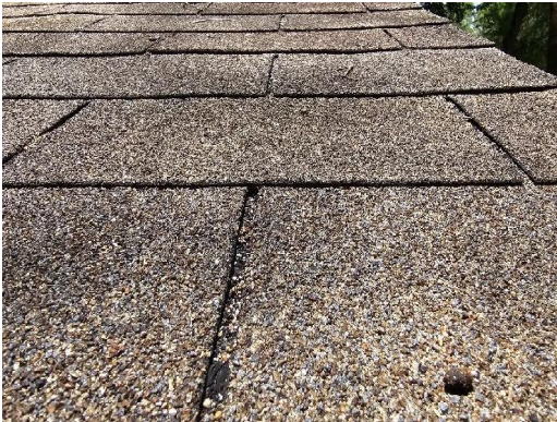
2612-1 Asphalt Shingle/Tar Typical Exterior Roof
